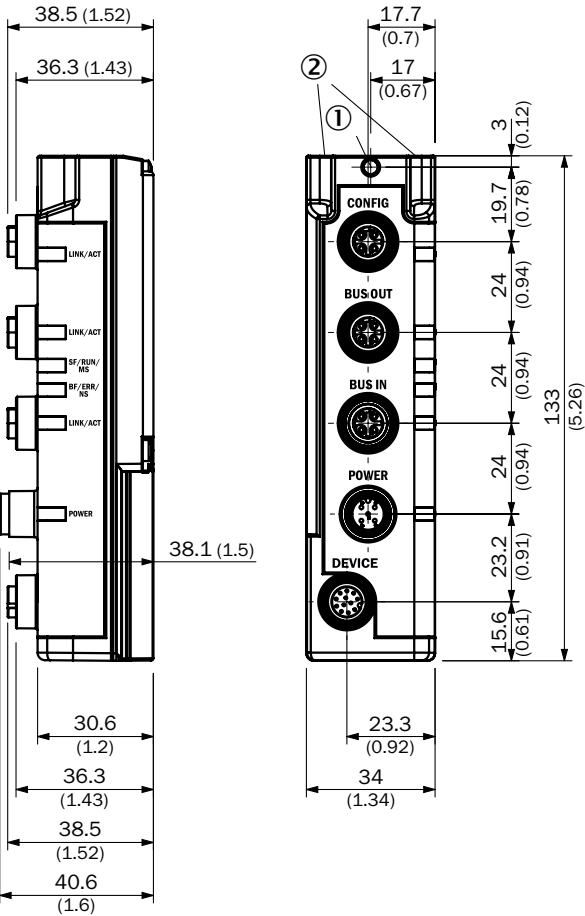
尺寸圖 PROFINET, ETHERCAT®, ETHERNET/IP
