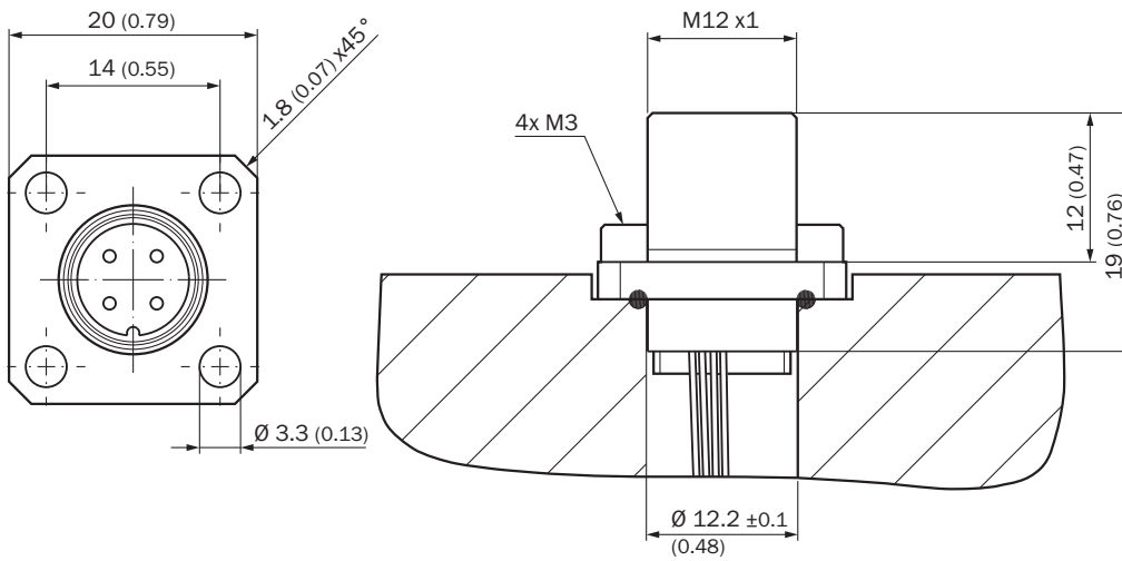
Dimensional drawing M12 connector type S/ flange - axial seal
