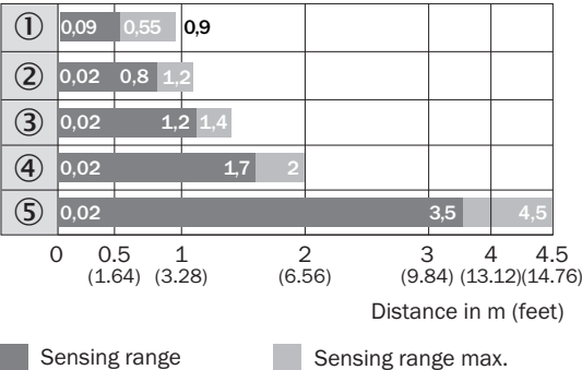
Sensing range diagram WLG4-3 with polarisation filter
