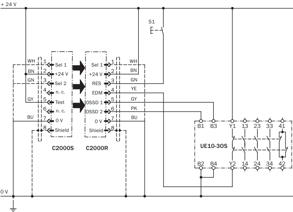
Connection diagram C2000 RES/EDM safety light curtain to UE10-30S safety relay
