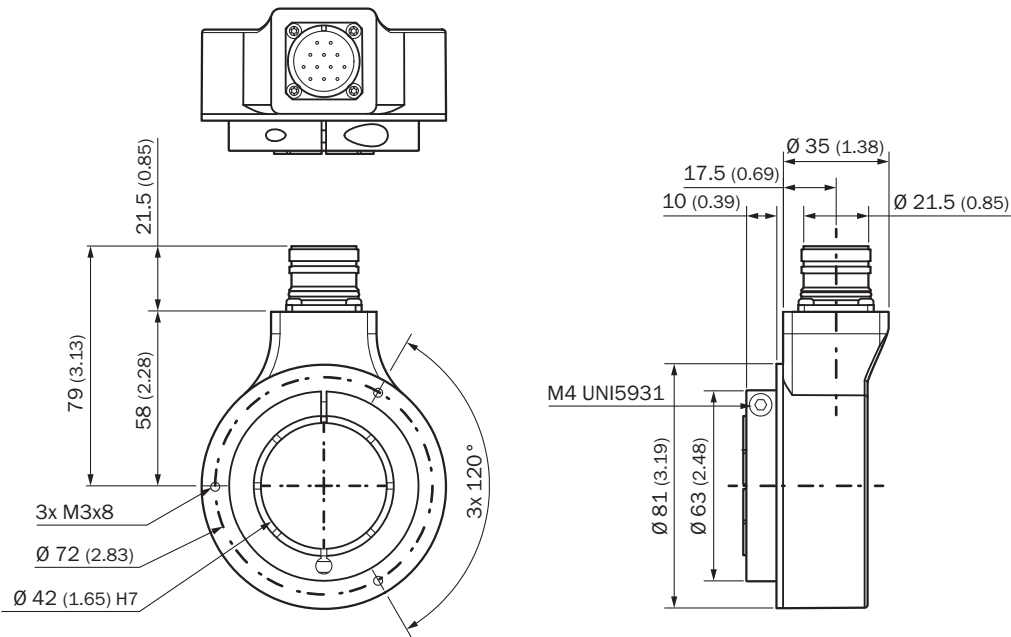
Dimensional drawing Bore hole size 42 mm, M23 male connector
