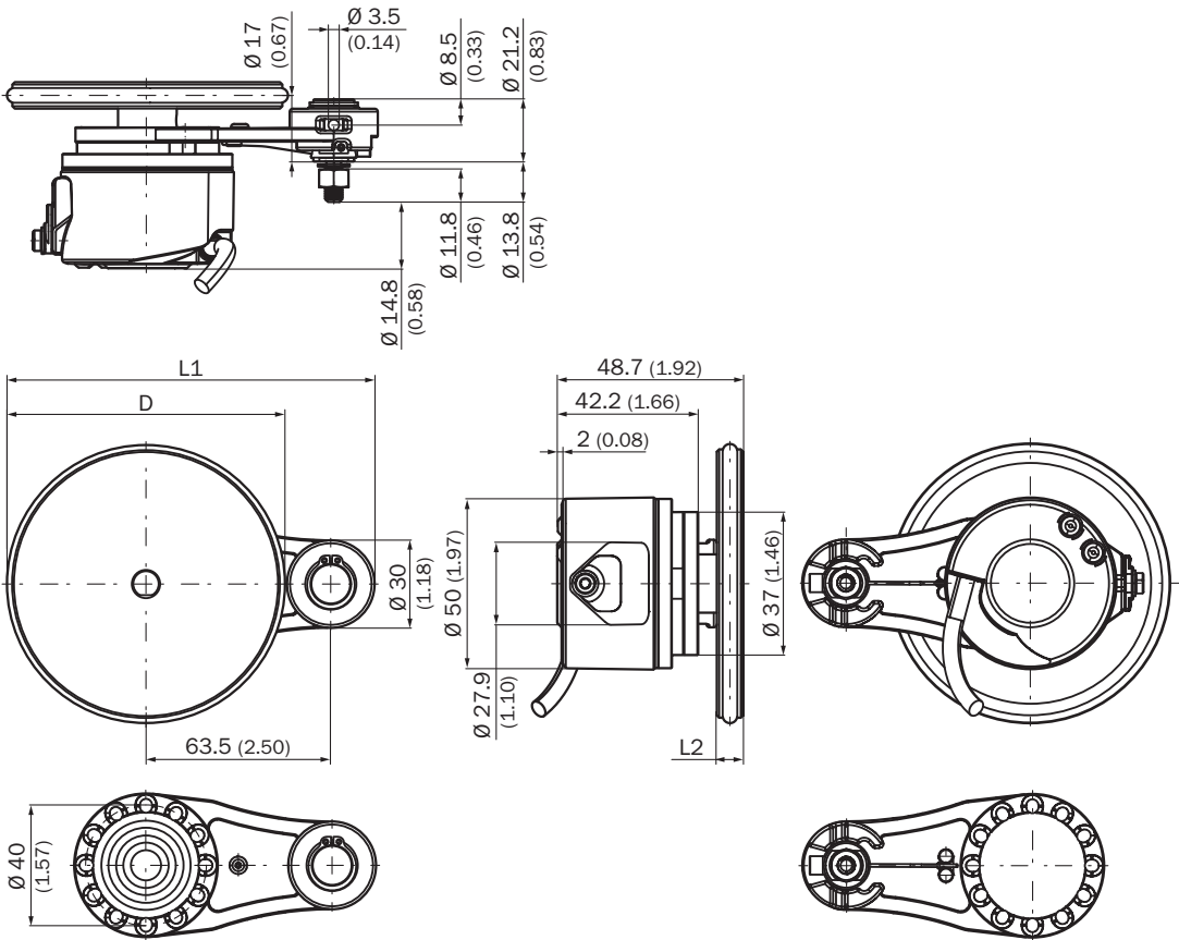
Dimensional drawing One measuring wheel, 63.5 mm spring arm, encoder on mounting side, cable
