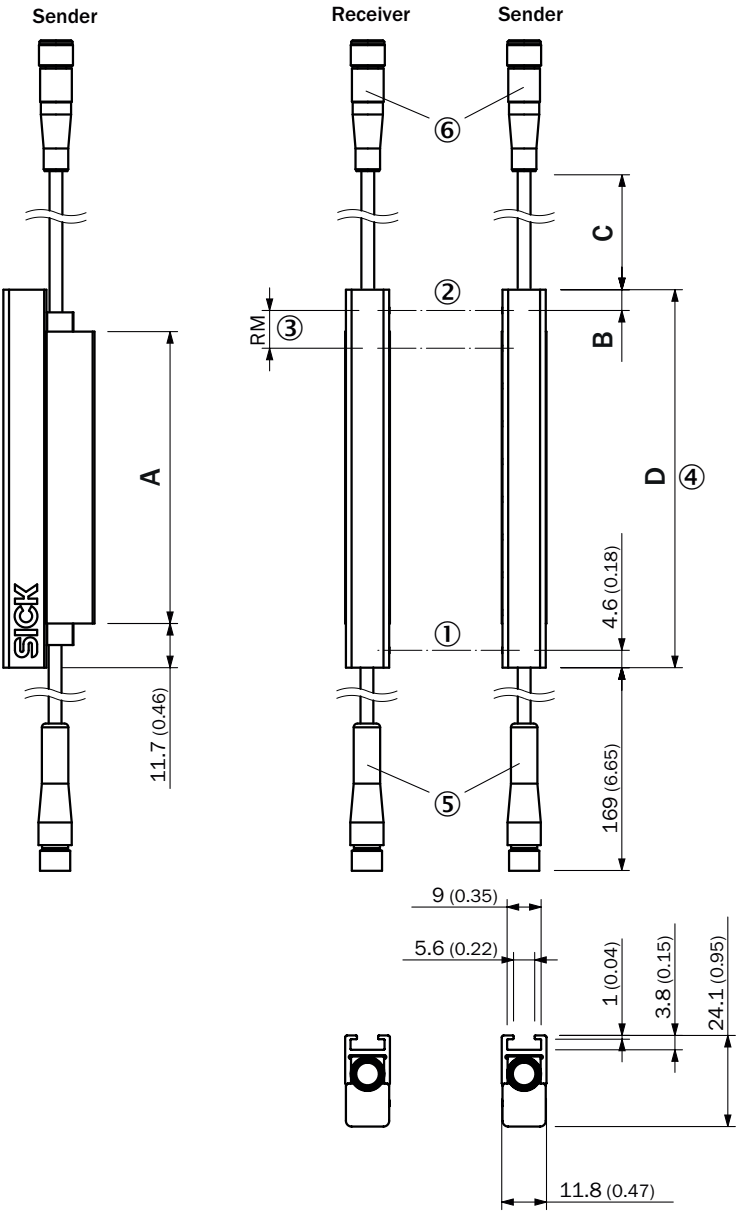
Dimensional drawing SLGxxx-xxxFxxxxxx
