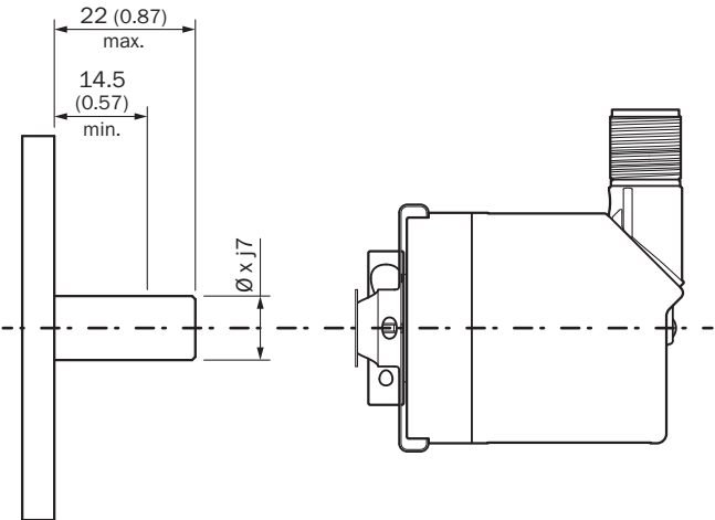
Attachment specifications
