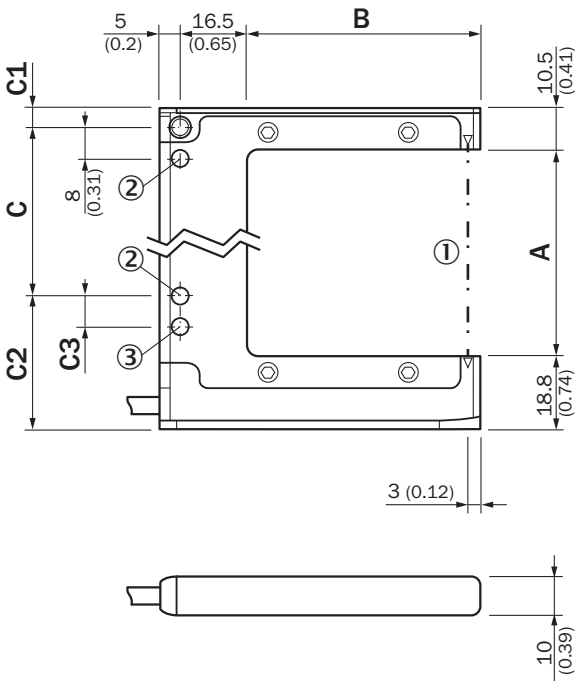
Dimensional drawing WFE-xxxxxxx1xx
