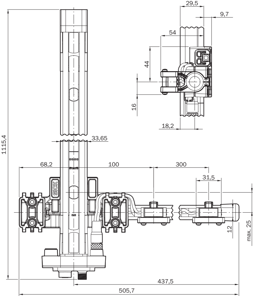
Dimensional drawing L muting right, active
