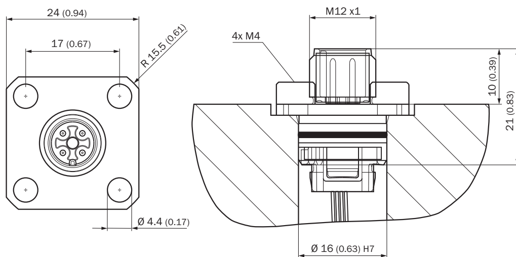
Dimensional drawing M12 connector type L/ flange - radial seal
