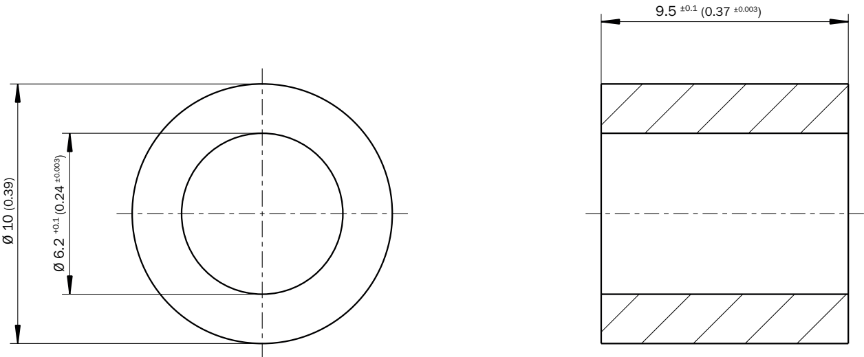
Dimensions in mm (inch)
