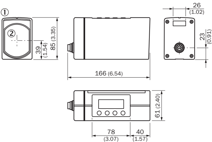
Dimensions in mm (inch) ① LC display ② Center of optical axis
