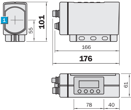
Dimensions in mm (inch) ① Center of optical axis
