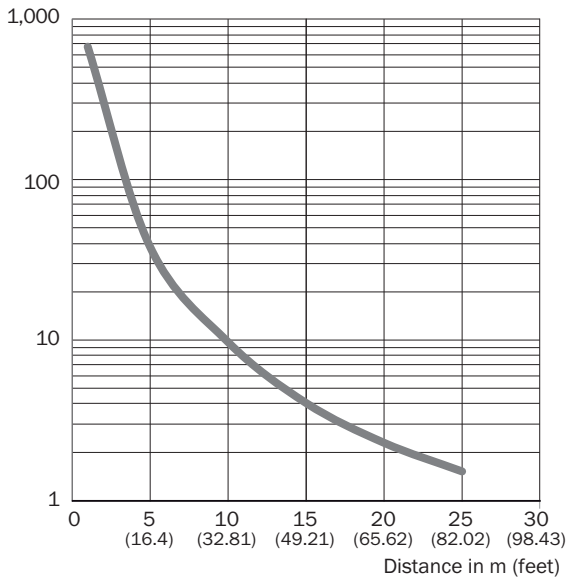
Operating reserve
