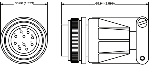
DOS-MS10-G Dimensions in mm (inch)
