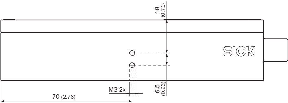
Dimensional drawing Side view with threaded holes for proximity sensors
