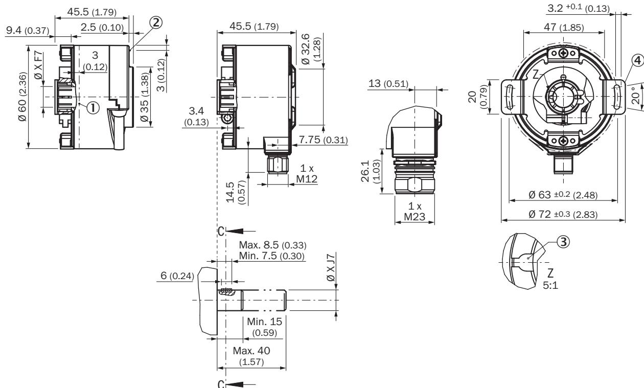
Dimensional drawing Through hollow shaft - safety system
