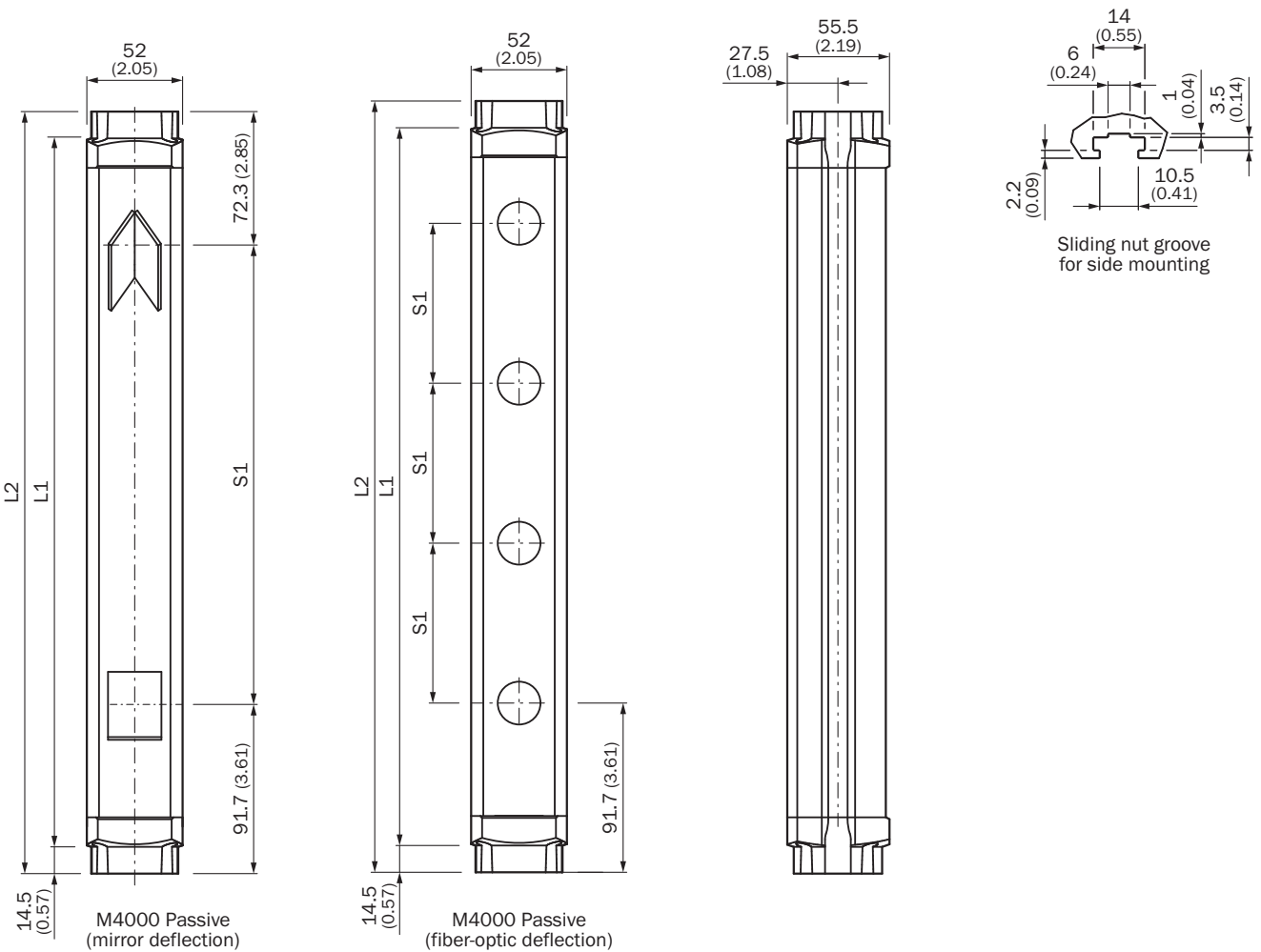
Dimensions in mm (inch) deflector unit
