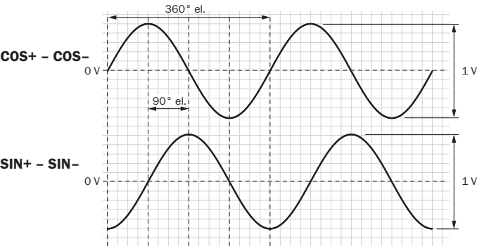
Diagrams Signal SIN/COS after differential generation
