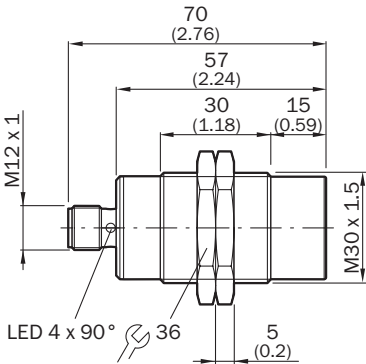
Dimensions in mm (inch)
