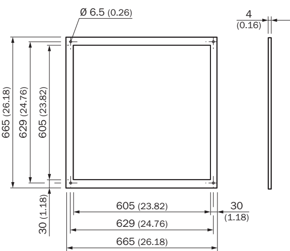
Dimensions in mm (inch)
