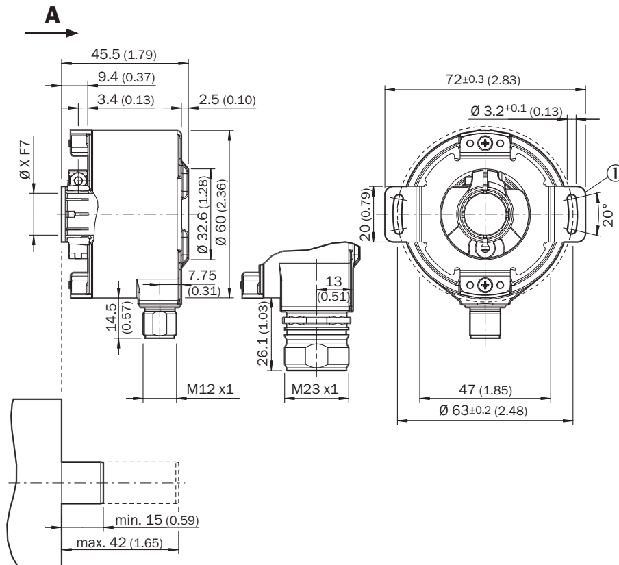
Dimensional drawing Blind hollow shaft, male connector - standard system
