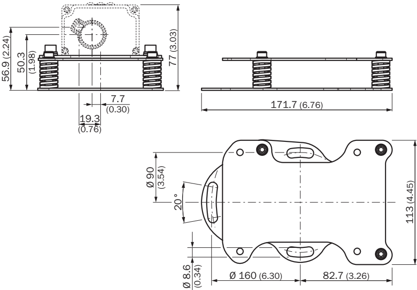
Dimensions in mm (inch)
