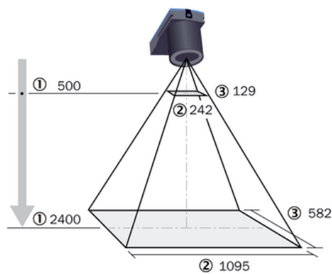
Fig. 2: Field of view of V2D8509R-xxxxxxxxxx, focal length: 25 mm, dynamic focus control
