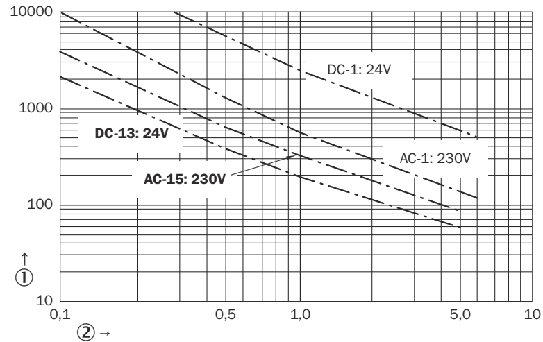
Figure 14: Electrical endurance of contacts 13/14 and 23/24
