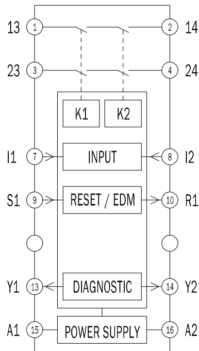
Figure 16: Internal circuitry
