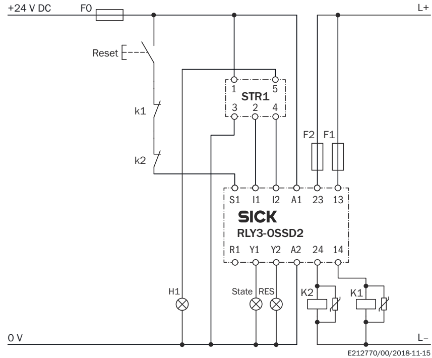
Figure 5: ReLy OSSD2 connection diagram, with restart interlock and external device monitoring (EDM)
