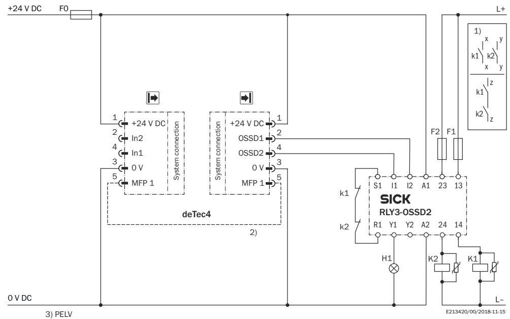
Figure 6: ReLy OSSD2 connection diagram, without restart interlock, with external device monitoring (EDM)
