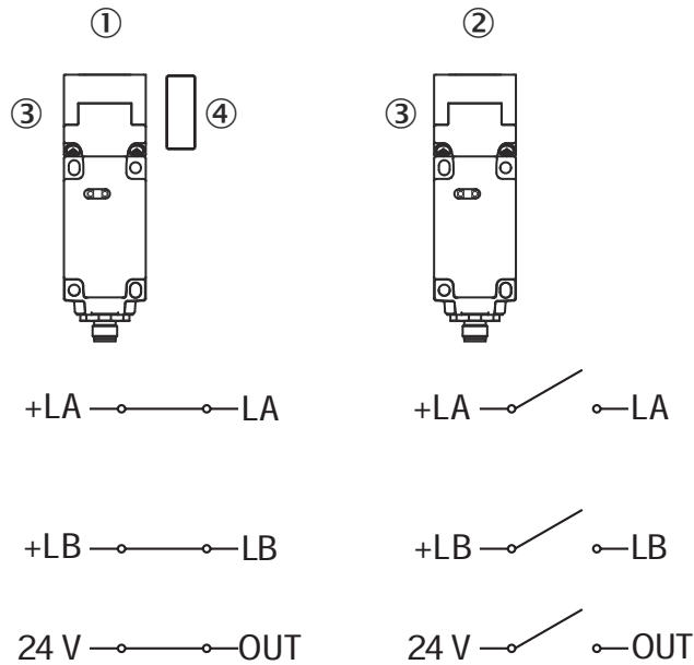
Figure 3: Switching behavior
