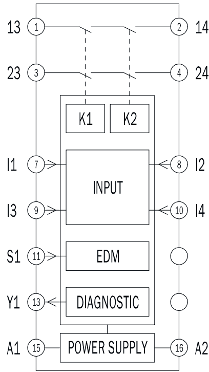
Figure 13: Internal circuitry
