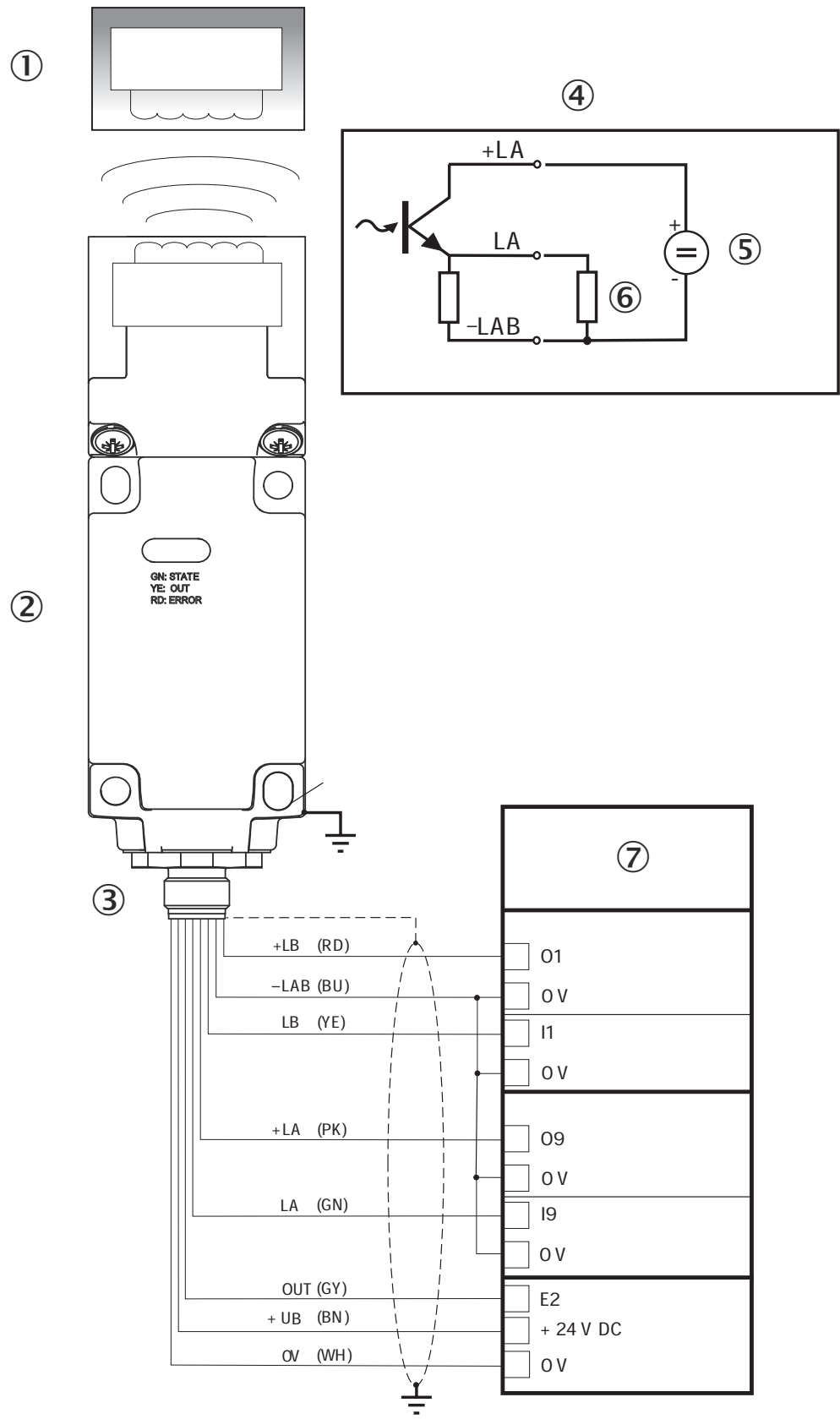
Figure 4: Connection example
