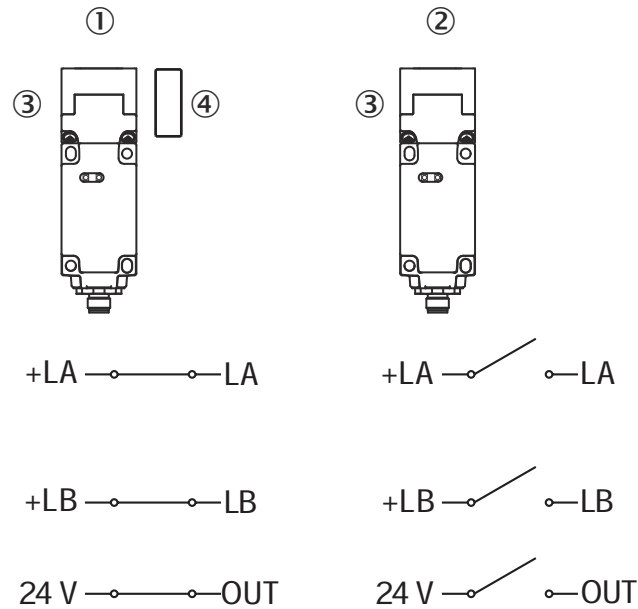
Figure 3: Switching behavior
