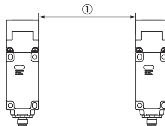
Figure 6: Minimum distance when several safety switches are mounted
