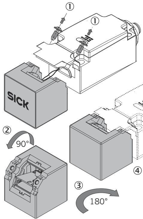
Figure 7: Changing the approach direction
