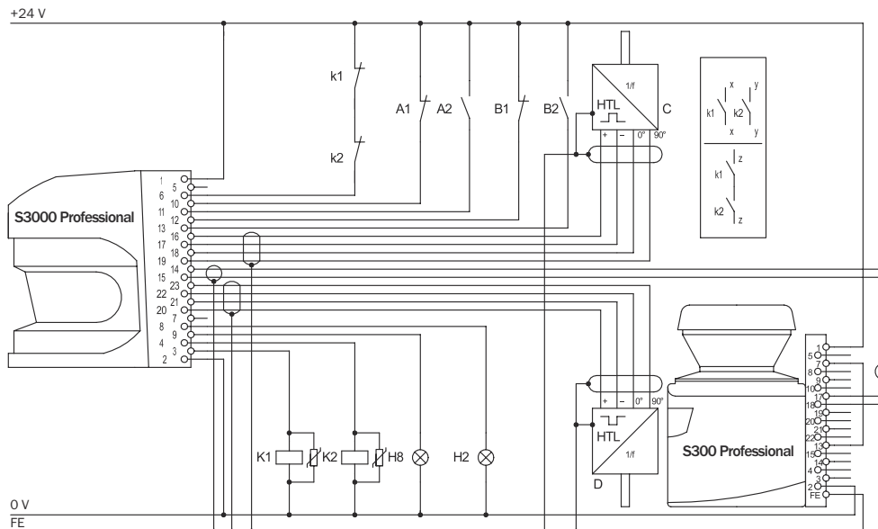
Figure 54: Connection diagram for monitoring case switching between an S3000 and an S300 using static and dynamic inputs
