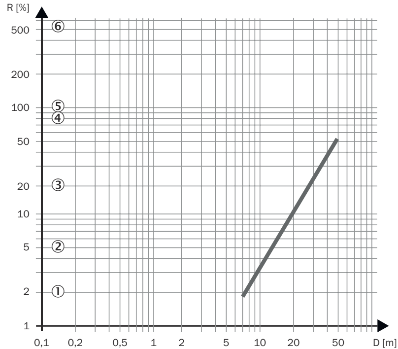
Figure 90: Diagram for scanning range of Long Range sensor head (maximum scanning range 7 m)
