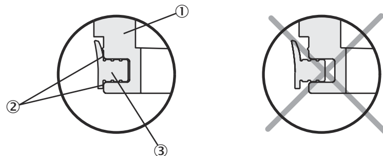
Figure 87: Depth for pressing in the seal
