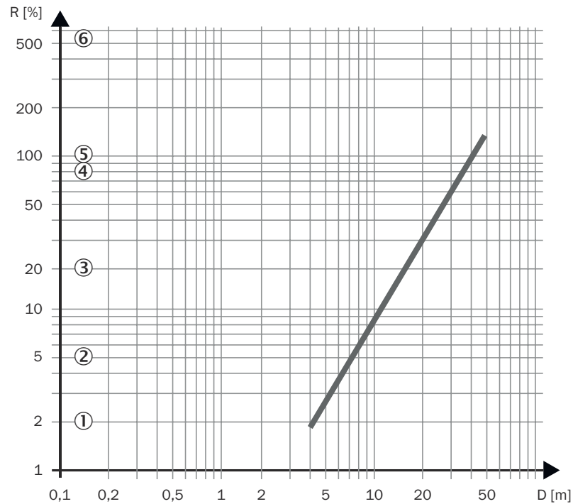
Figure 88: Diagram for scanning range of Short Range sensor head (maximum scanning range 4 m)
