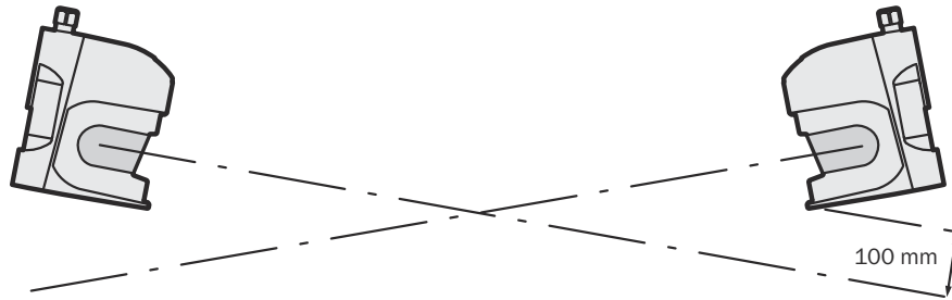
Figure 21: Mounting opposite
