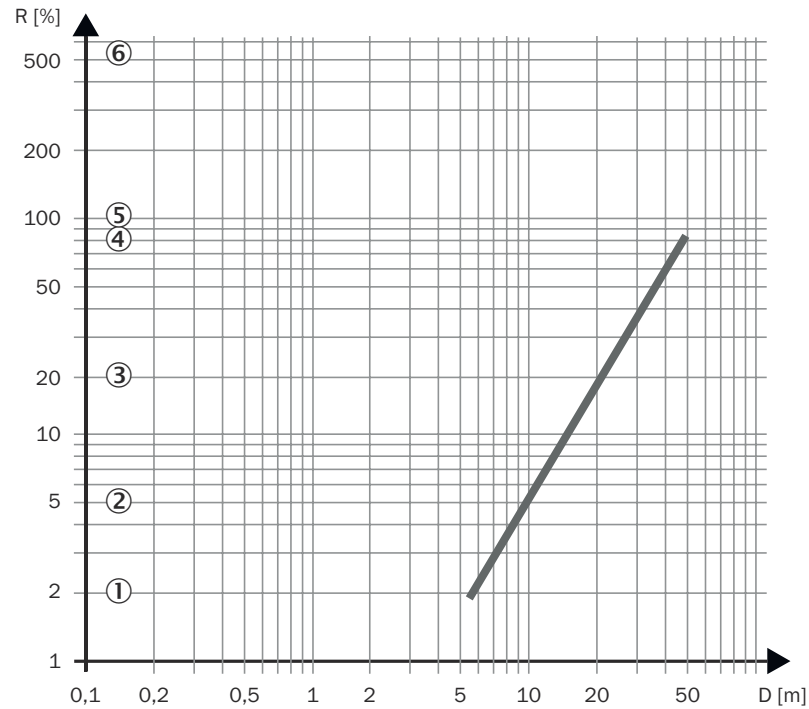
Figure 89: Diagram for scanning range of Medium Range sensor head (maximum scanning range 5.5 m)
