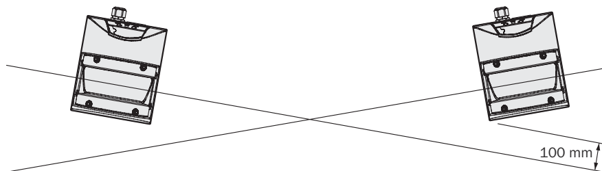
Figure 24: Mounting crosswise
