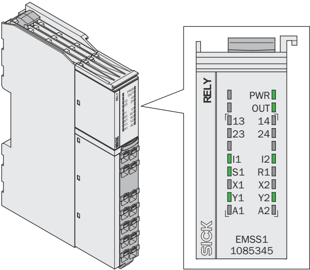
Illustration 2 : LED
