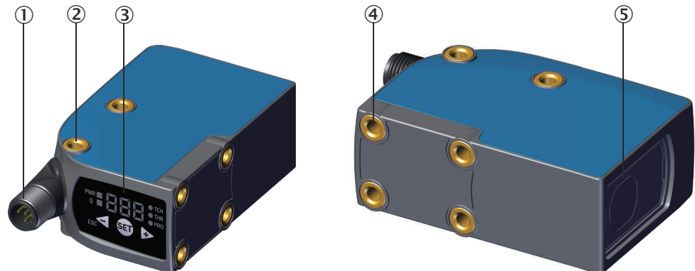
Figure 3: KTX Prime light emission short housing side
