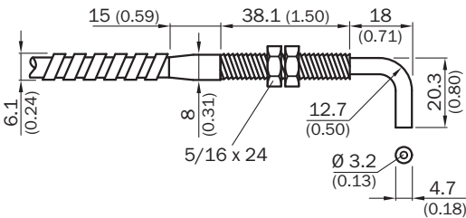
Dimensional drawing LISTA32900, LBSTA32900, LISTA321800
