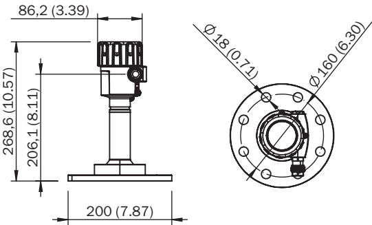
Dimensions in mm (inch) LBR-xxCFABOHAAX
