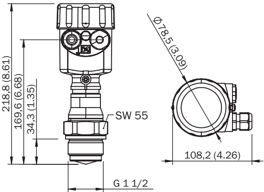
Dimensions in mm (inch) LBR-xxTTCAMHKA
