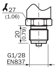
Dimensions in mm (inch)
