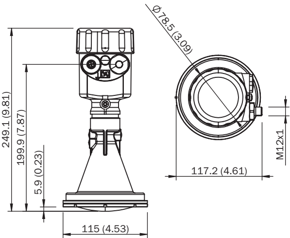
Dimensions in mm (inch) LFR-xxBXXCBHKKX
