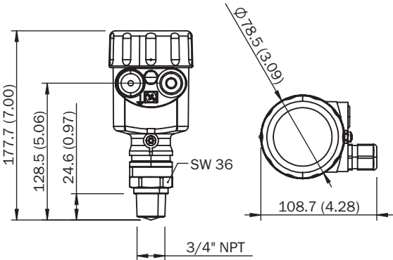
Dimensions in mm (inch) LFR-xxTTBAJHKAX
