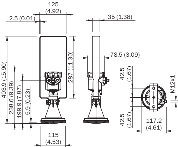
Dimensions in mm (inch) LFR-xxBXDCBHKXX
