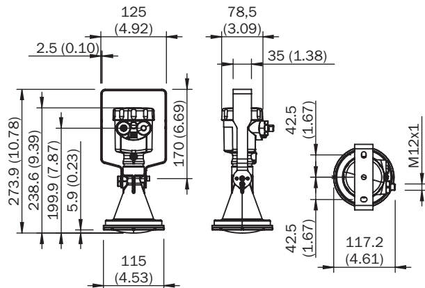
Dimensions in mm (inch) LFR-xxBXCCBHKXX
