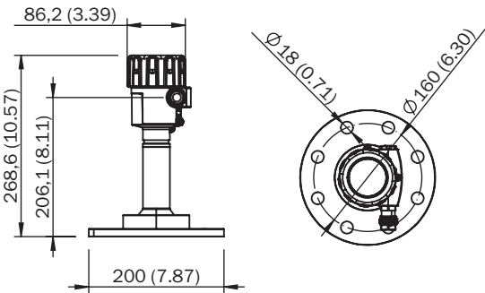
Dimensions in mm (inch) LBR-xxCFABOHAA
