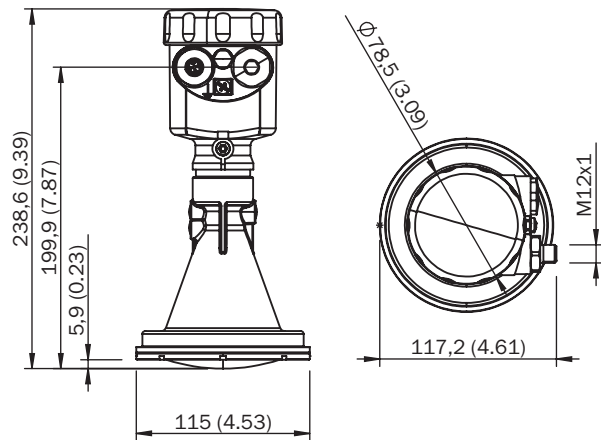
Dimensions in mm (inch) LBR-xxBXXCBHKXX
