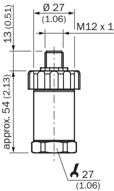
Dimensional drawing Housing with circular plug-in connector M12 x 1
