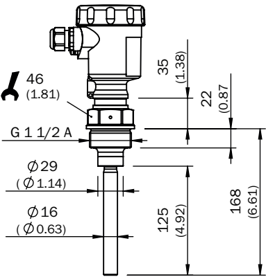
Dimensional drawing LBV311 threaded version G 1 ½ A
