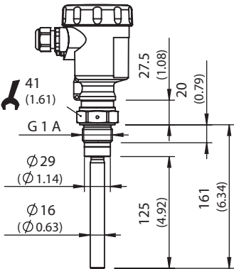
Dimensional drawing LBV311 threaded version G 1 A
