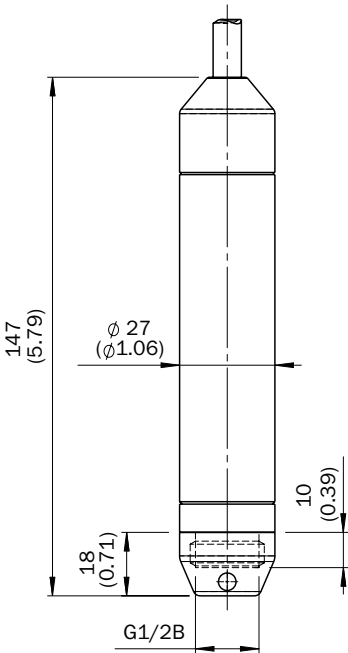
Dimensional drawing Enhanced variant with FEP cable (immersion depth up to 100 m)
