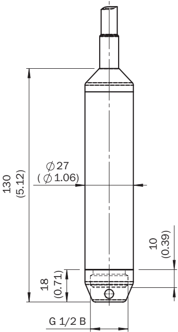
Dimensional drawing Enhanced variant with PUR cable (immersion depth up to 100 m)
