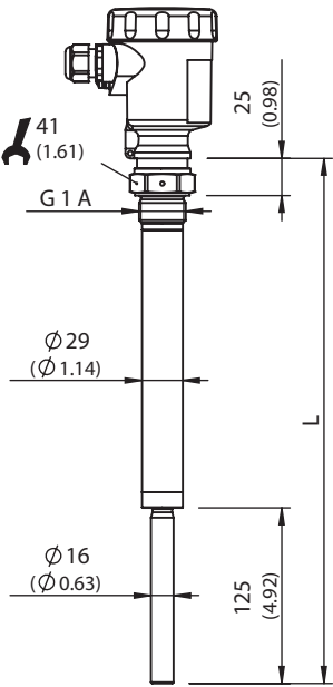
Dimensional drawing LBV331 threaded version G 1 A
