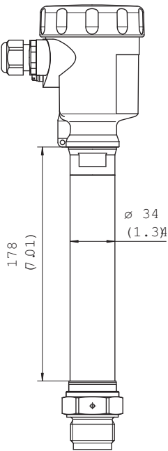
Dimensional drawing Temperature adapter
