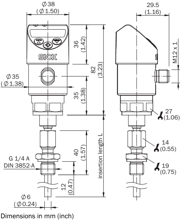
Dimensional drawing Compression fitting G 1/4 A
