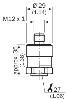
Dimensional drawing Housing with circular connector M12 x 1, IP67
