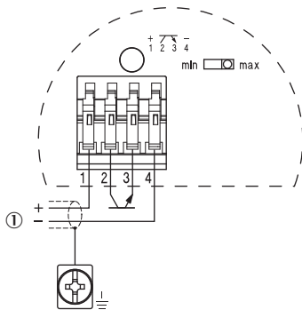
Connection diagram Transistor connection diagram
