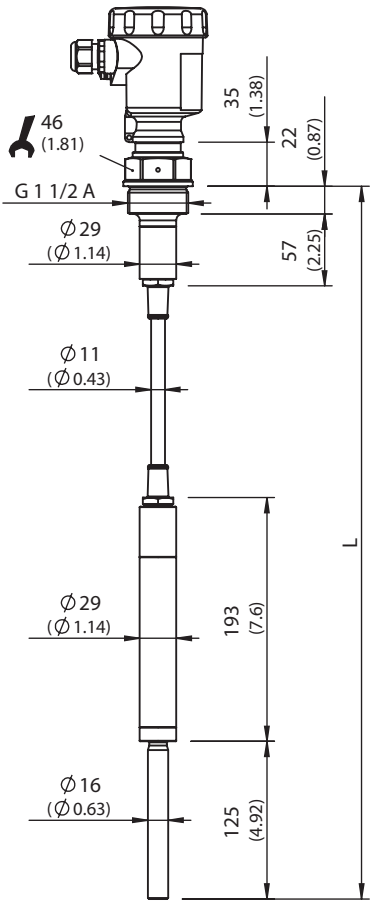
Dimensional drawing LBV321 threaded version G 1 ½ A
