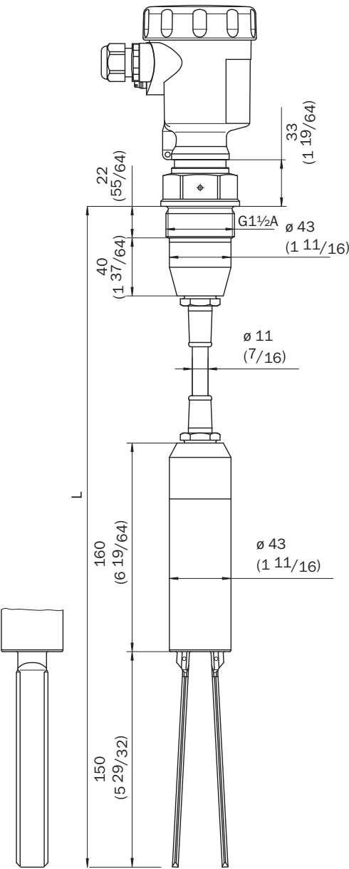
Dimensional drawing LBV320 with PUR suspension cable, threaded version G 1½ A (DIN ISO 228/1)
